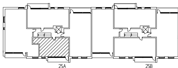
ORIENTERINGSPLAN PLAN 2
