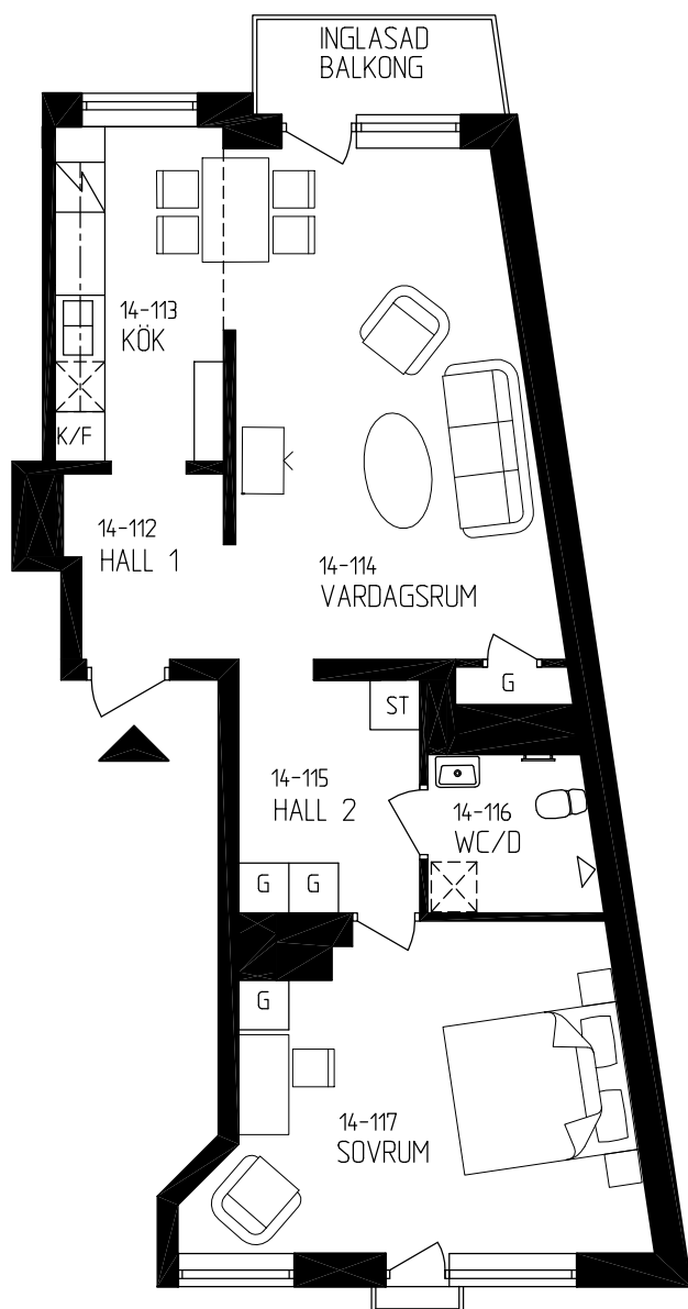
BOTTENPLAN
