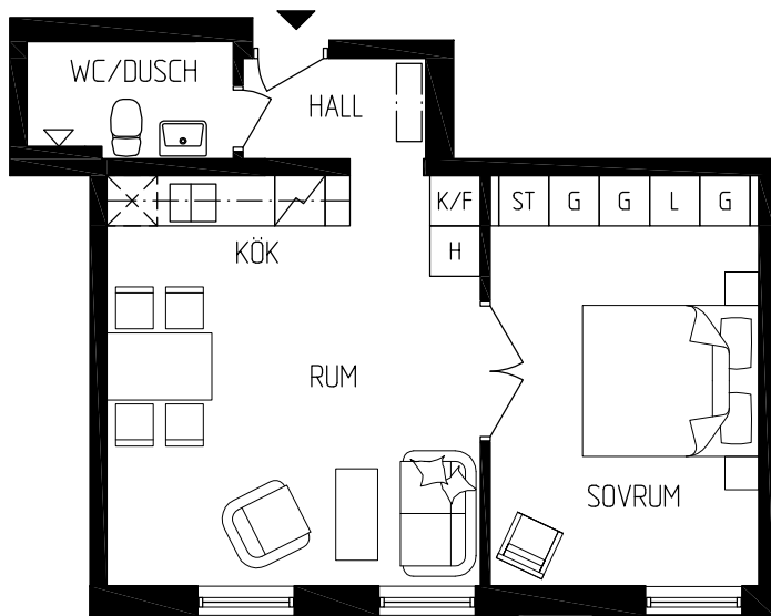
PLAN 1 TR
